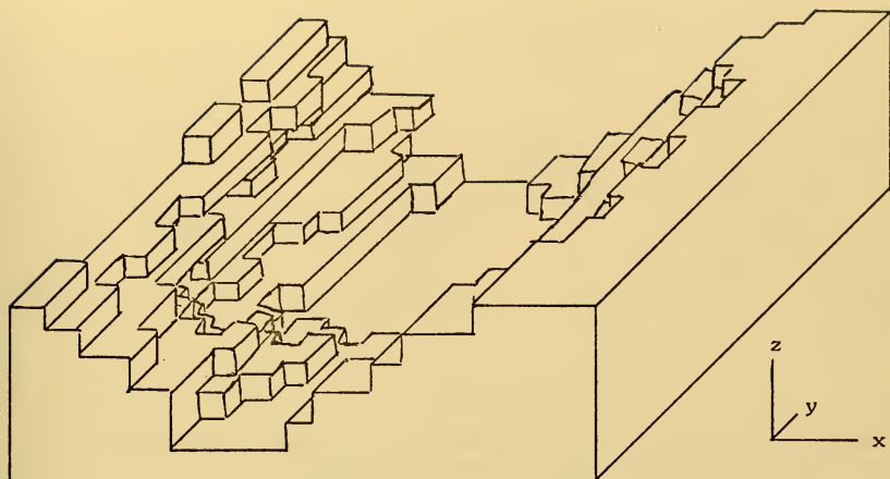
Figure 24. Microstate 310 of an Initially Perfect Surface at 10,000^{\circ}\text{K} . (a) Lines bordering atoms and clusters of atoms are parallel and perpendicular to the \langle 100 \rangle direction.
